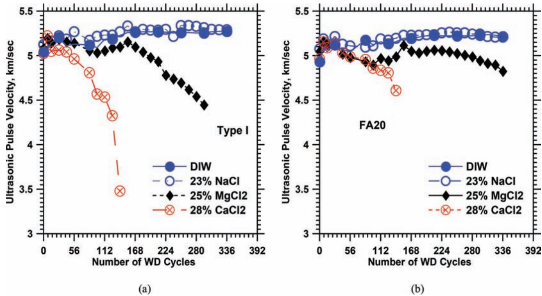
Figure 4.27 UPV for (a) Type I, and (b) FA 20 mixtures exposed to WD regime.
