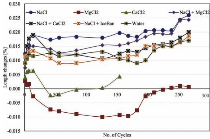
Figure 4.10 Length changes (%) of FA 20 test samples subjected to W/D cycles.
