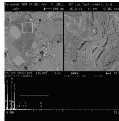
(d) MSH formation in Type I specimen subjected to IceBan and NaCl solution
