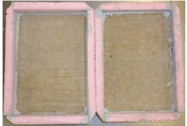
Figure B.3 Appearance of the specimens that were subjected to scaling test in the presence of the combination of sodium chloride and calcium chloride (NaCl + CaCl 2 ) after 100 cycles of exposure (left – Type I; right – FA).
