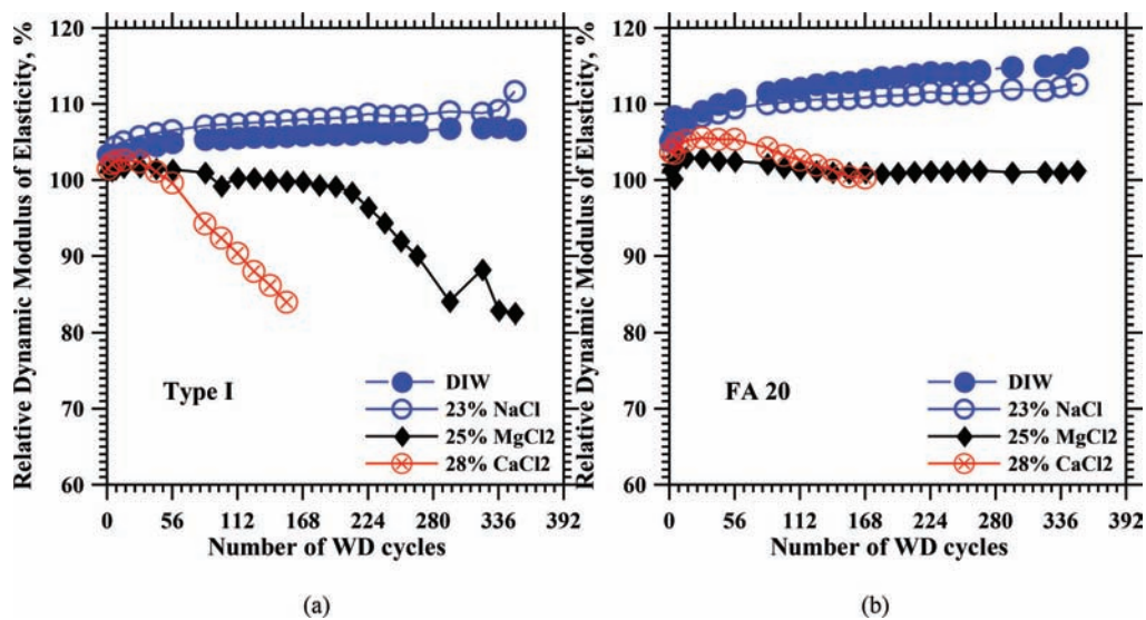
Figure 4.4 RDME values for (a) Type I, and (b) FA 20 specimens exposed to W/D regime.
