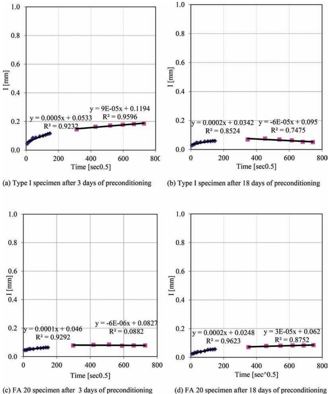
Figure C.2 Absorption of concrete specimens when subjected to the solution of 25% MgCl_2 : (a) Type I specimen after 3 days of preconditioning, (b) Type I specimen after 18 days of preconditioning, (c) FA 20 specimen after 3 days of preconditioning, (d) FA 20 specimen after 18 days of preconditioning.
