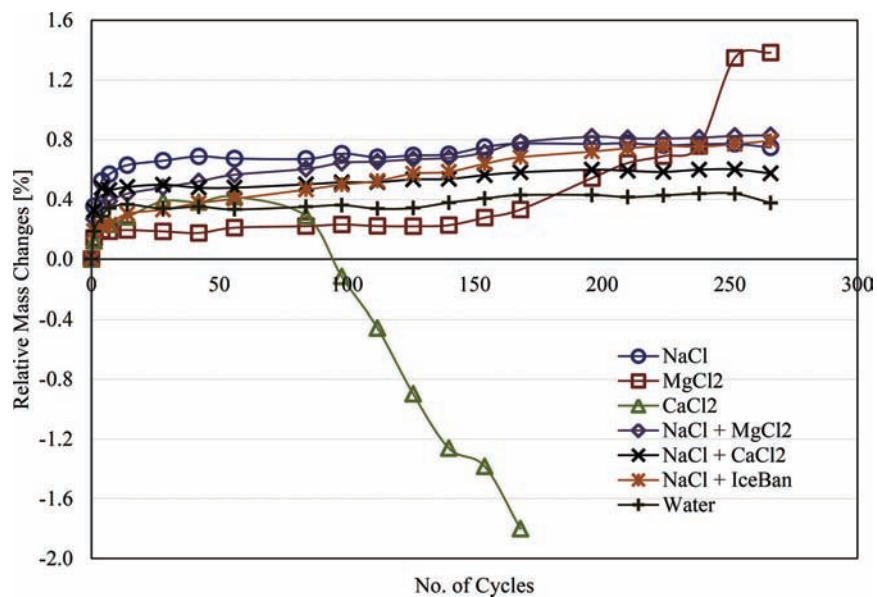
Figure 4.15 Relative mass changes (%) of Type I test samples subjected to W/D cycles.
