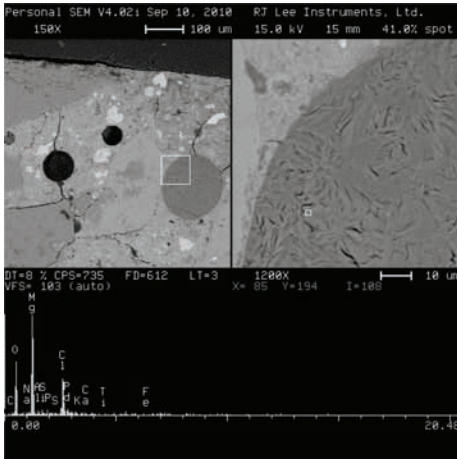
(a) Magnesium oxychloride formation in FA specimen subjected to MgCl_2 and W/D cycles
