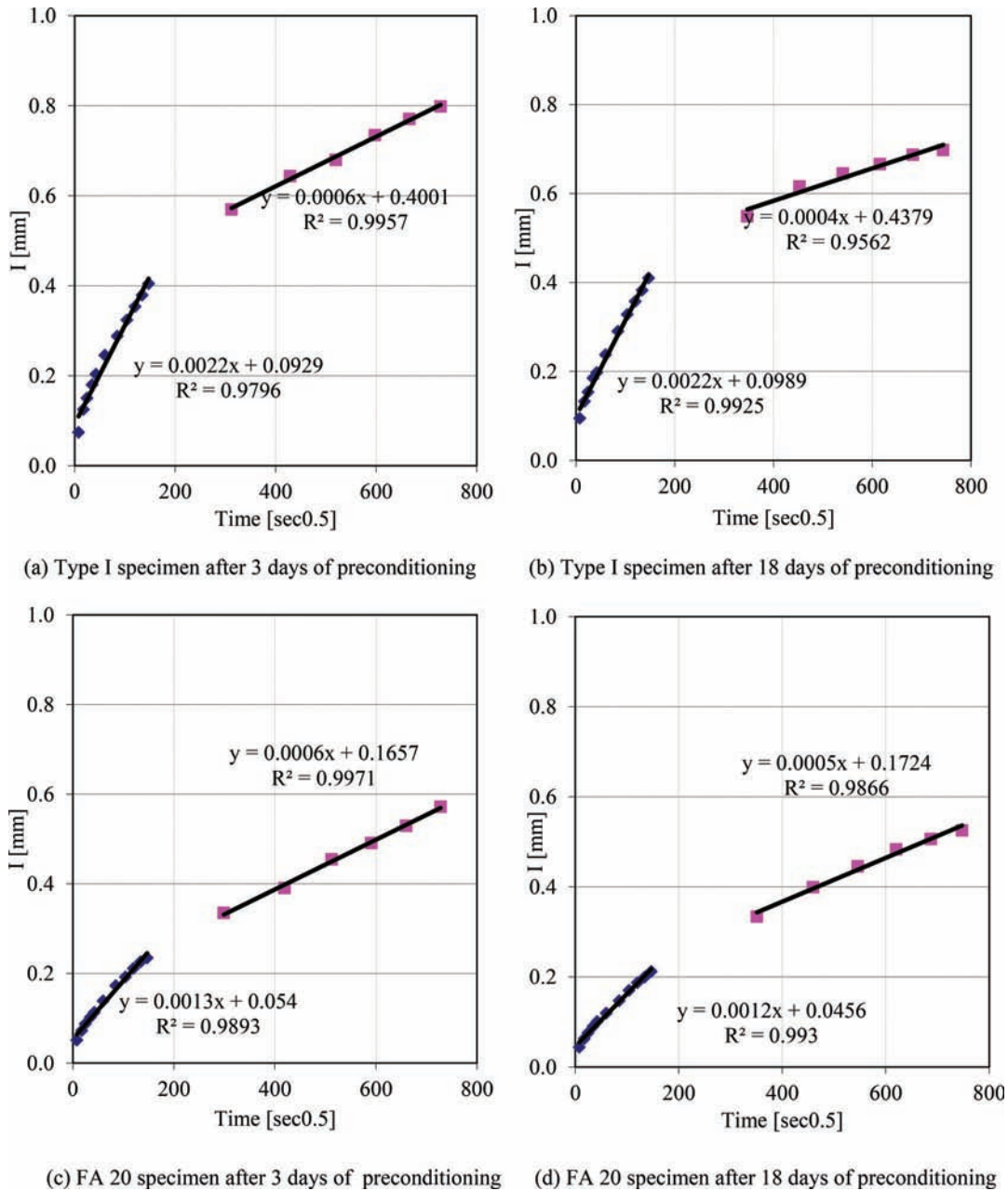
Figure C.1 Absorptions of concrete specimens when subjected to 23% NaCl: (a) Type I specimen in 3 days preconditioning, (b) Type I specimen in 18 days preconditioning, (c) FA 20 specimen in 3 days preconditioning, (d) FA 20 specimen in 18 days preconditioning.
