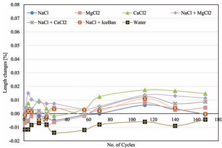
Figure 4.12 Length changes (%) of FA 20 test samples subjected to F/T cycles.
