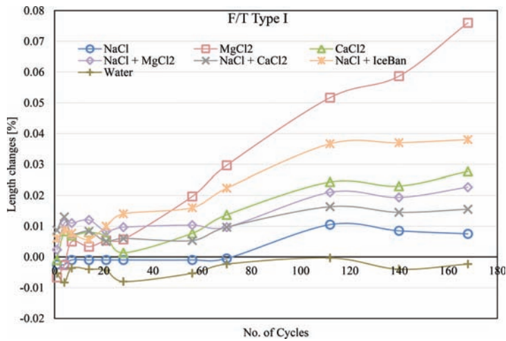
Figure 4.11 Length changes (%) of Type-I test samples subjected to F/T cycles.
