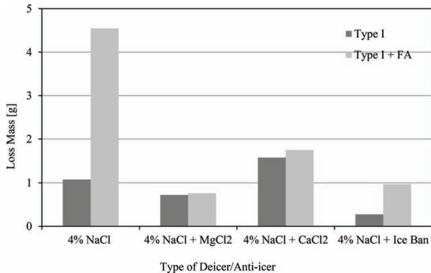
Figure 4.25 Mass losses of concrete specimens subjected to different deicing solutions.
