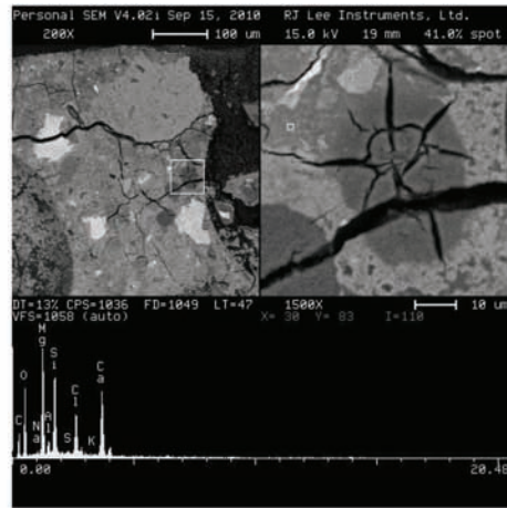
(b) Brucite formation in FA specimen subjected to IceBan and NaCl solution
