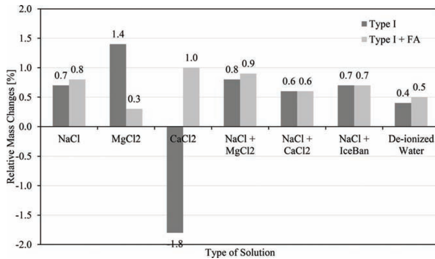
Figure 4.19 Relative mass changes (%) of concrete samples subjected to 266 W/D cycles.
