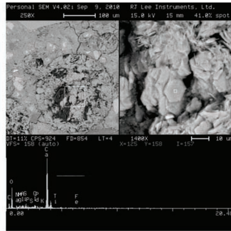
(b) Deposits of Ca(OH) 2 in Type I specimen subjected to CaCl 2 and W/D cycle
