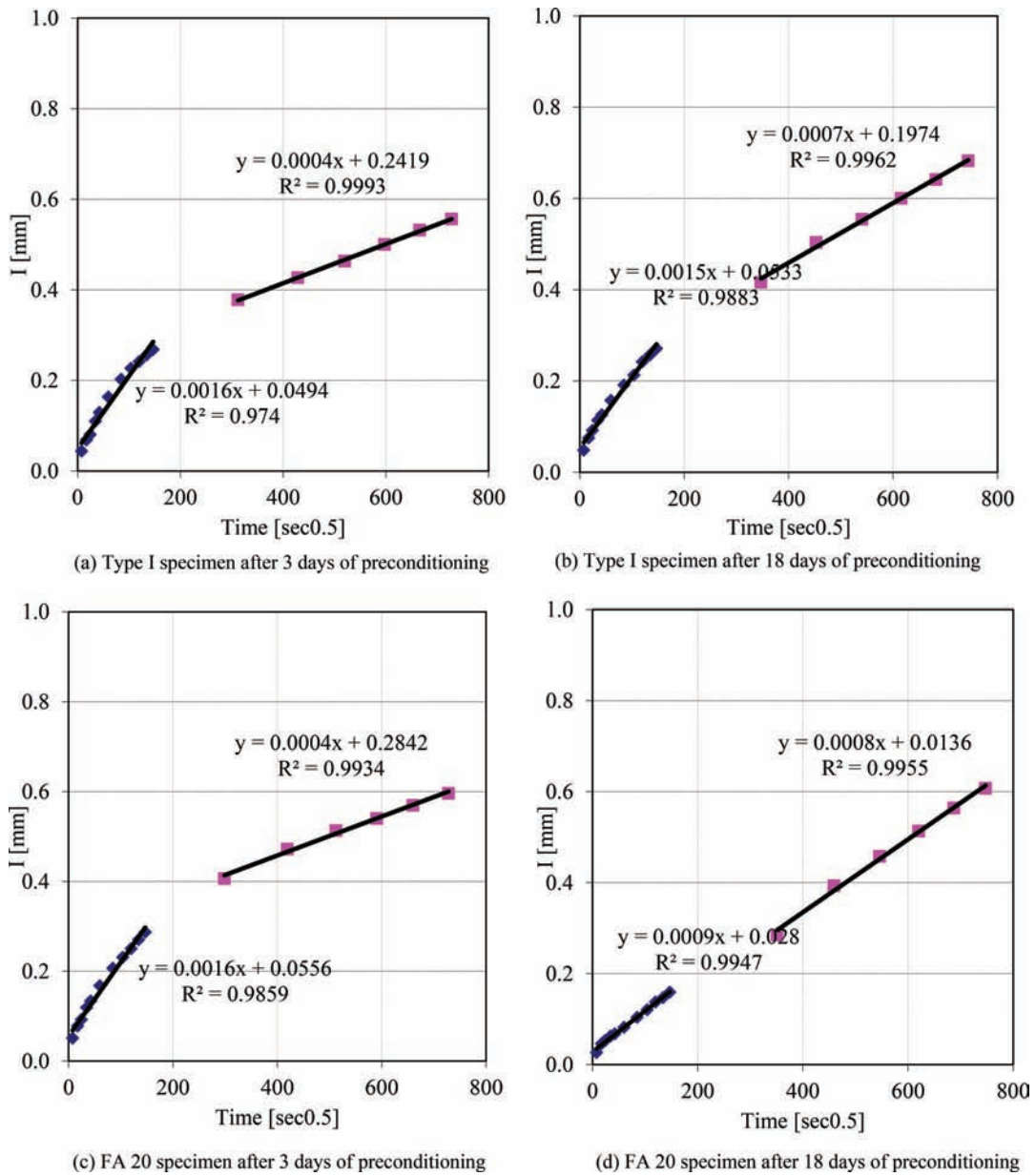
Figure C.4 Absorption of concrete specimens when subjected to Deionized Water: (a) Type I specimen after 3 days of preconditioning, (b) Type I specimen after 18 days of preconditioning, (c) FA 20 specimen after 3 days of preconditioning, (d) FA 20 specimen after 18 days of preconditioning.
