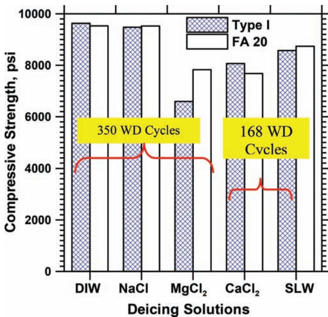
Figure 4.26 Compressive strengths for specimens exposed to different deicers under WD regime.
