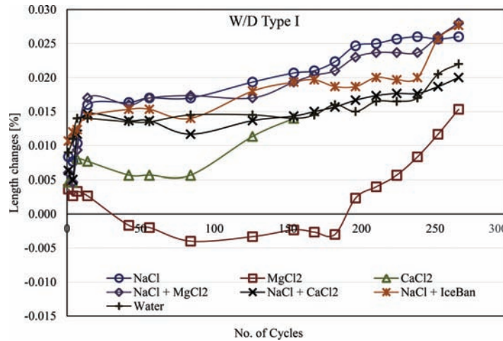
Figure 4.9 Length changes (%) of Type-I test samples subjected to W/D cycles.
