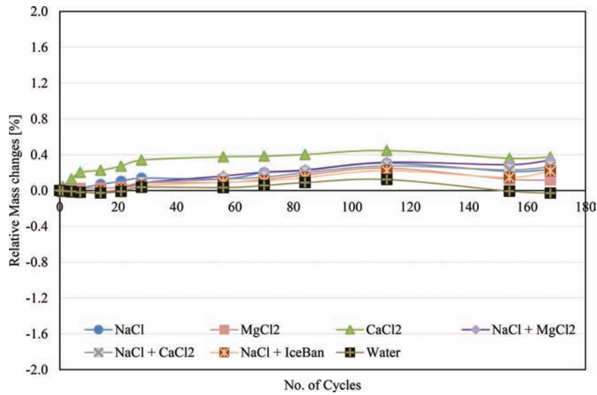
Figure 4.18 Relative mass changes (%) of FA 20 test samples subjected to F/T cycles.
