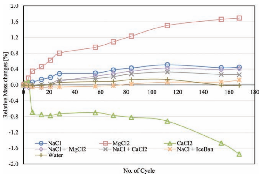
Figure 4.17 Relative mass changes (%) of Type I test samples subjected to F/T cycles.
