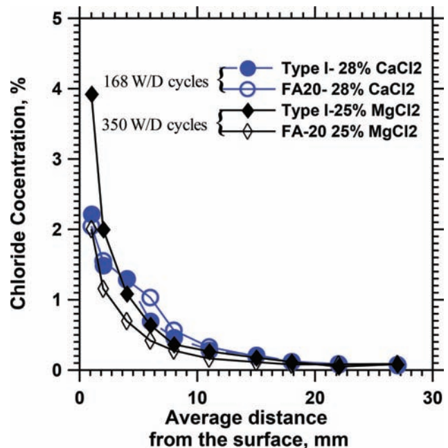
Figure 4.28 Penetration of acid soluble chlorides in specimens after 168 W/D cycles in CaCl 2 solution and 350 W/D cycles in MgCl 2 solution.
