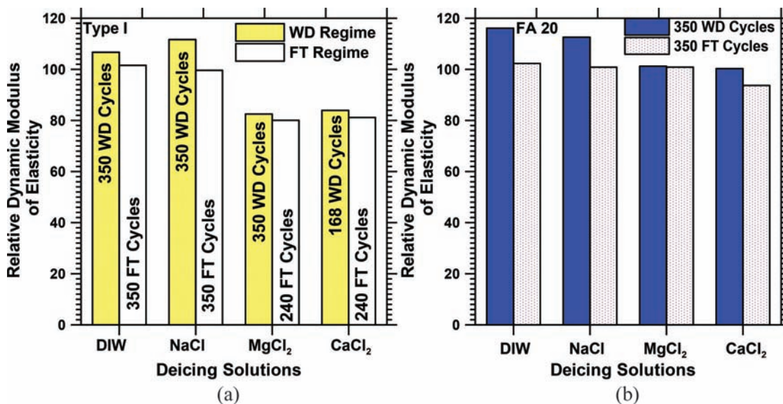
Figure 4.6 RDME values for (a) Type I and (b) FA 20 specimens subjected to WD and FT exposure.
