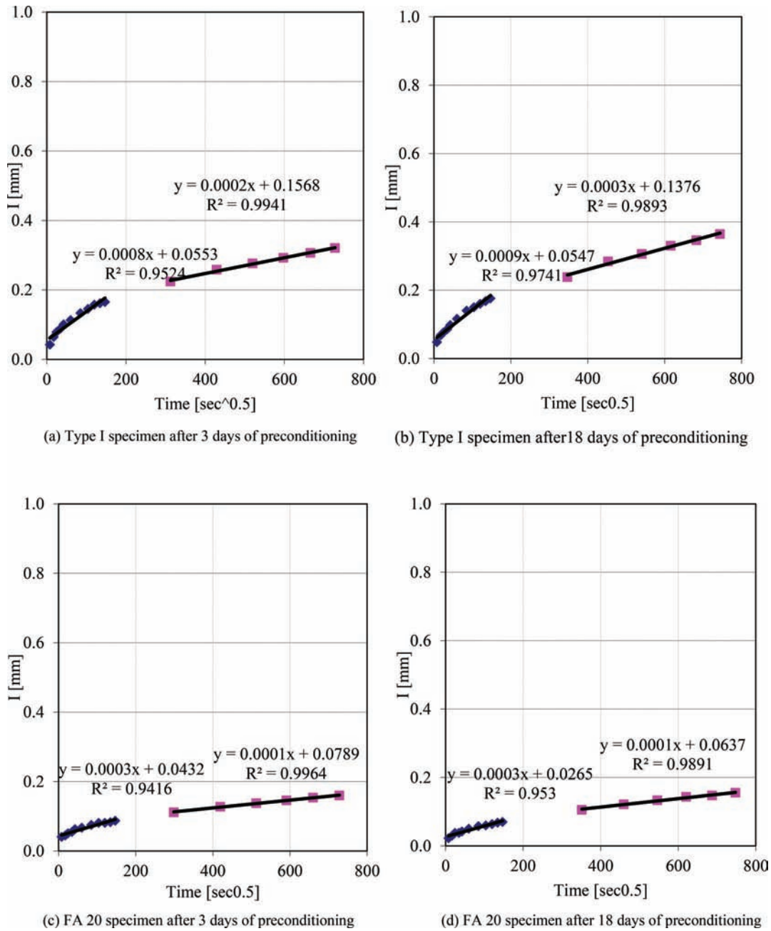
Figure C.3 Absorption of concrete specimens when subjected to 28% CaCl 2 : (a) Type I specimen after 3 days of preconditioning, (b) Type I specimen after 18 days of preconditioning, (c) FA 20 specimen after 3 days of preconditioning, (d) FA 20 specimen after 18 days of preconditioning.
