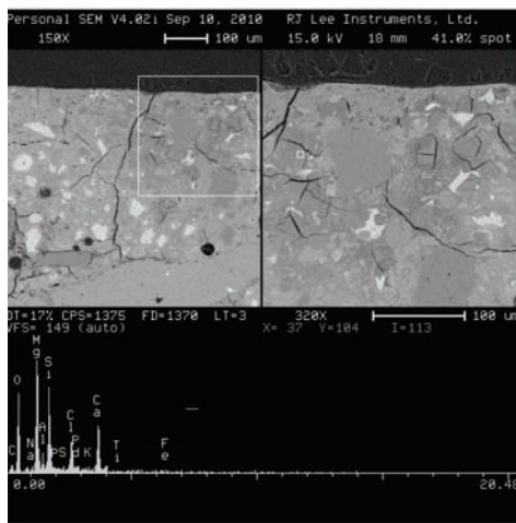
(c) MSH formation in type I specimen subjected to MgCl 2 and W/D cycles
