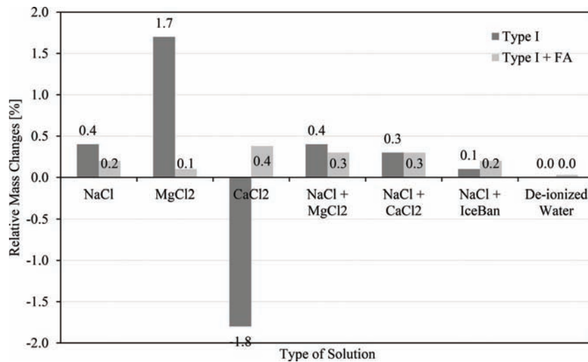
Figure 4.20 Relative mass changes (%) of concrete samples subjected to 266 F/T cycles.
