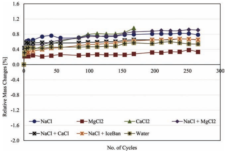
Figure 4.16 Relative mass changes (%) of FA 20 test samples subjected to W/D cycles.
