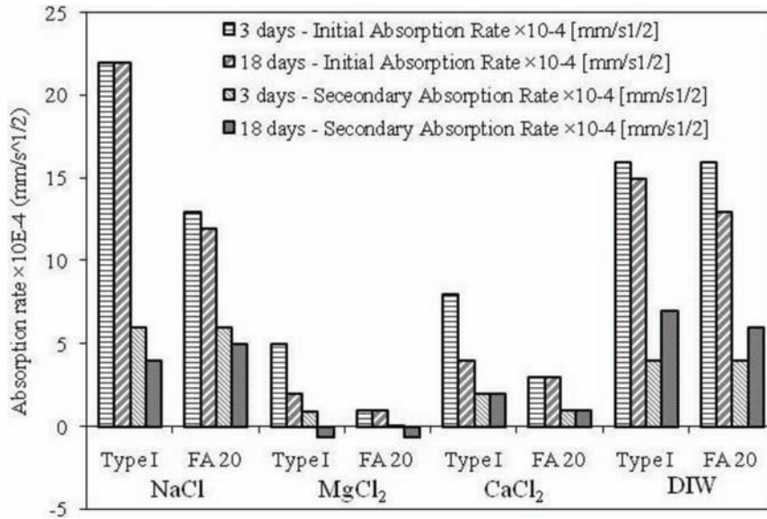
Figure 4.21 The Initial and the secondary rates of absorption for specimens exposed to different deicing solutions.
