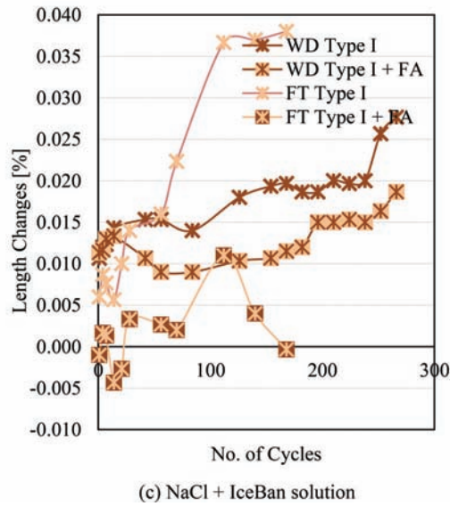
Figure 4.8 Length changes (%) of test specimens subject to different exposure condition: (a) NaCl + MgCl 2 solution (b) NaCl + CaCl 2 solution, and (c) NaCl + Ice Ban solution.
