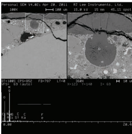
(c) Brucite formation in Type I specimen subjected to IceBan and NaCl solution
