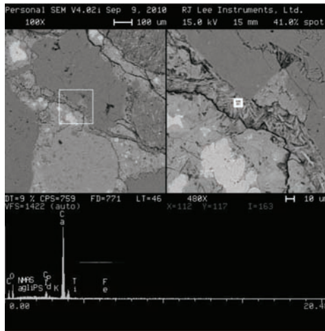
(a) EDX peaks shows the tracing of calcium oxychloride in Type I specimen subjected to 28 % CaCl 2 and W/D cycle
