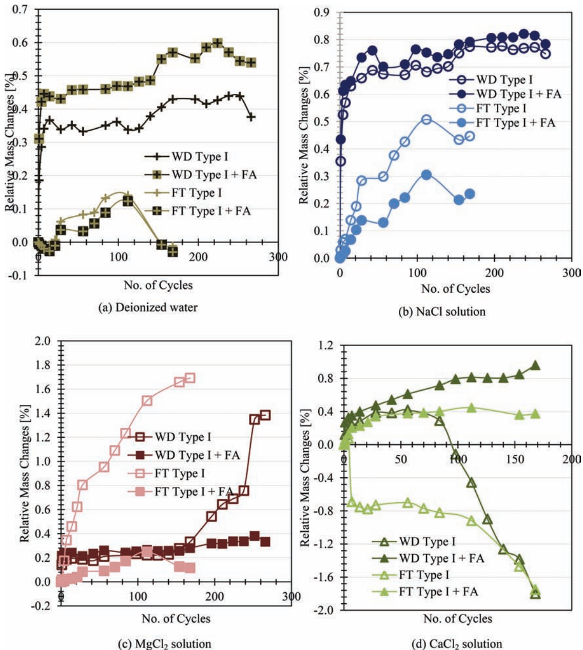
Figure 4.13 Mass changes (%) of samples subjected to different exposure condition (a) Deionized water, (b) NaCl solution, (c) MgCl_2 solution, and (d) CaCl_2 solution.
