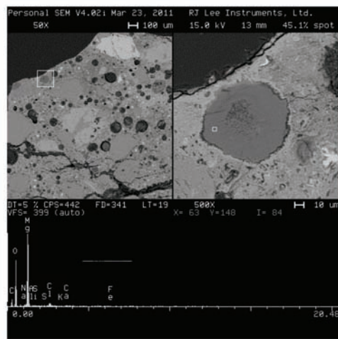
(d) Brucite formation in type I specimen subjected to MgCl 2 and FT cycles
