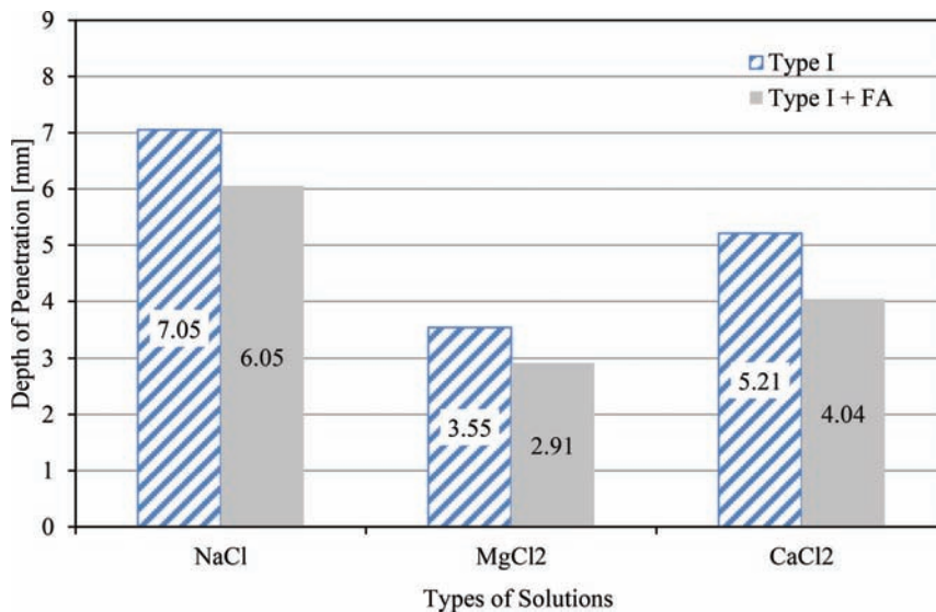
Figure 4.22 Average depth of chloride ion penetration for 3 days preconditioned specimens.
