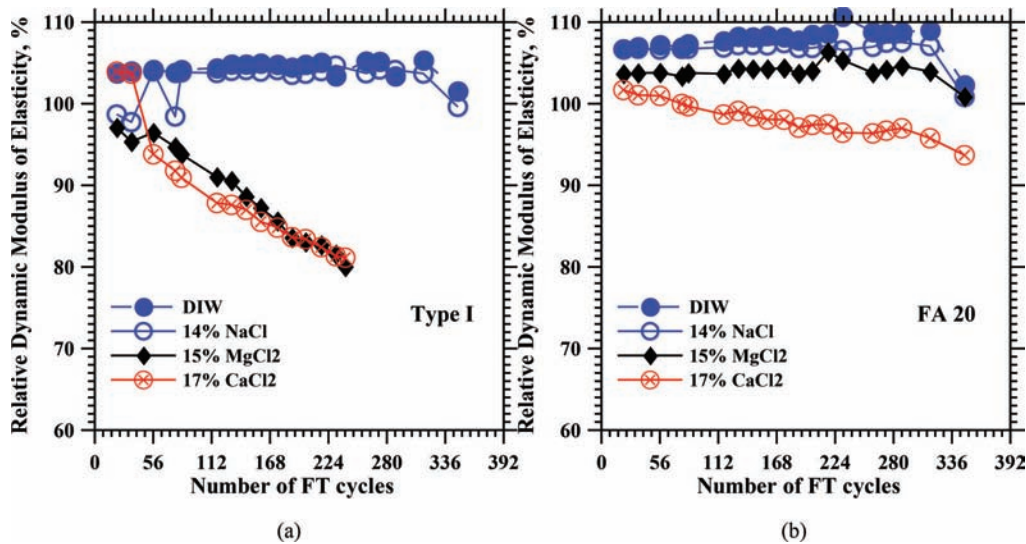
Figure 4.5 RDME Values for (a) Type I and (b) FA 20 specimens subjected to FT regime.
