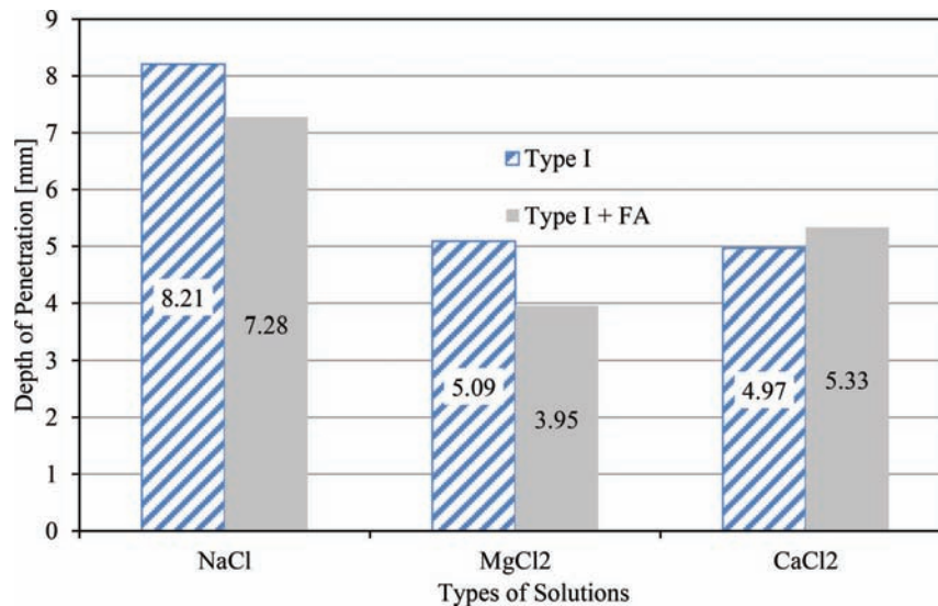
Figure 4.23 Average depth of chloride ion penetration for 18 days preconditioned specimens.
