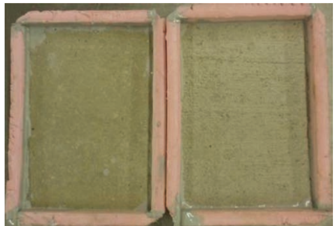
Figure B.4 Appearance of the specimens that were subjected to scaling test in the presence of the combination of sodium chloride and Ice Ban ® after 100 cycles of exposure (left – Type I; right – FA).
