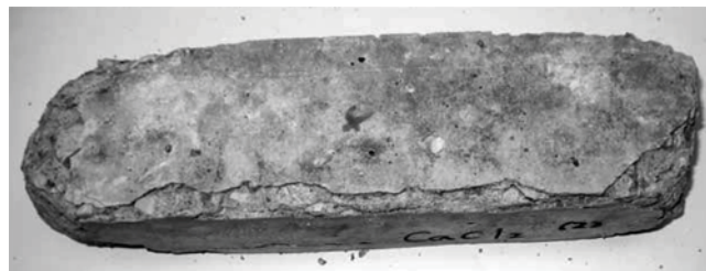
Fig. 9—Specimen subjected to 10 weeks of exposure to 6.04 molal ion concentration solution of CaCl 2 .
